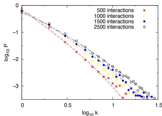
Fig. 4. Log-log plots of the degree distributions of the networks obtained by random removal of links from 2008 simulation data. The number of interactions left on the networks are indicated. The data are fitted by formula given by Eq. (1) using \gamma = 2.4 and letting k_0 and k_c varied.
