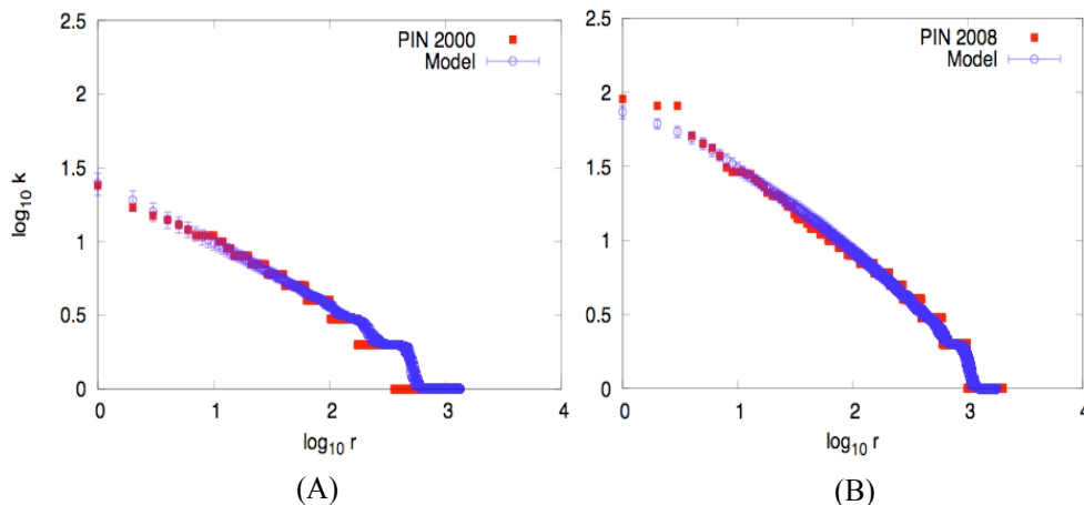
Fig. 2. Log-log plots of the dependence of degree k of the nodes on their rank r . The figure compares the results from the model and the 2000 experimental data (A) and 2008 experimental data (B).
