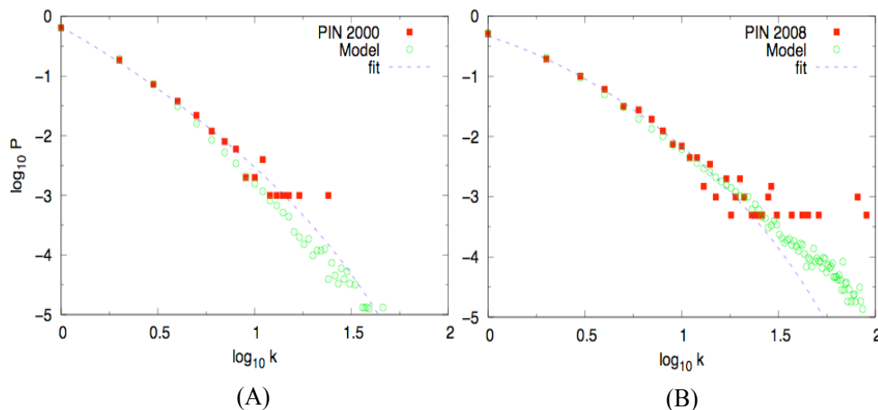
Fig. 1. Log-log plots of the degree distribution P(k) obtained by the duplication-divergence model and from experimental data for the protein interaction network of S. cerevisiae . (A) Comparison between the model and experimental data collected by Uetz et al. [5] in year 2000. (B) Comparison between the model and experimental data collected by Yu et al. [7] in year 2008. The data of the model and experiments are shown in open circles and filled squares, respectively, as indicated. Experimental data are fitted by the formula given by Eq. (1) (dashed line) with \gamma = 2.4 , k_c = 15 , k_0 = 0.4 for the data in 2000 and \gamma = 2.4 , k_c = 16 , k_0 = 1.5 for the data in 2008.
