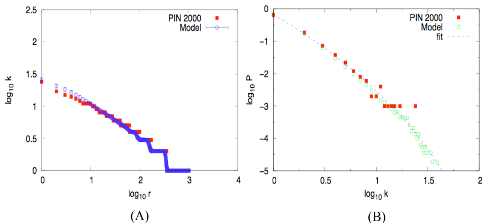
Fig. 3. Log-log plots of order-rank dependence (A) and degree distribution (B) for the networks obtained by random removal of links from the simulation data for year 2008. The model is compared to experimental data (filled squares) for year 2000 as indicated.
