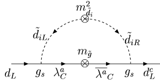
Fig. 8. Diagram giving mass to quark d which does not appear in the superpotential, \tilde{g} is the gluino, \tilde{d}_i , i = 1, 2 , is the down-squark.
