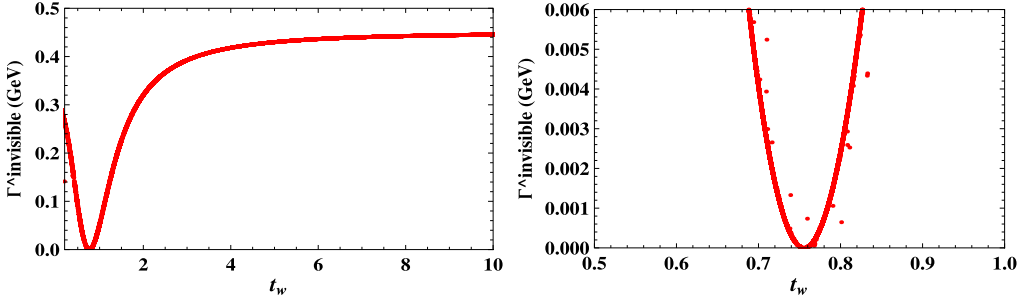
Fig. 10. The invisible decay rate of Z^\mu into the massless of the doubly charged Higgs bosons by studying random scan over the parameter space w = 10^3\text{--}10^5 GeV, t_w = 0\text{--}10 and t_v = 0\text{--}100 , v'_\rho = 246 GeV.
