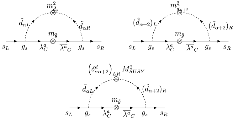
Fig. 9. Diagram giving mass to s -quark which does not appear in the superpotential, \tilde{g} is the gluino, \tilde{s}_i and \tilde{b}_i , i = 1, 2 , are the squark s and sbottom, respectively.
