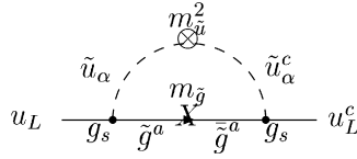
Fig. 7. Diagram giving mass to up quark which does not appear in the superpotential, \tilde{u} is the up-squark.
