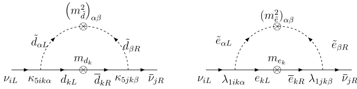
Fig. 4. Diagrams giving masses to electron’s and muon’s neutrinos which do not appear in the superpotential, \tilde{e} is the selectron and \tilde{d} is the down-squark and the label \alpha = 1, 2 .
