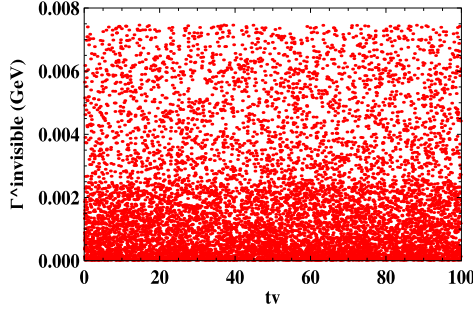
Fig. 11. The invisible decay rate of Z^\mu into the massless doubly charged Higgs bosons as the function of t_v by studying random scan over the parameter space w = 10^3\text{--}10^5 GeV, t_w = 0.68\text{--}0.8 , v'_\rho = 246 GeV.
