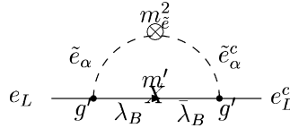
Fig. 1. Diagram giving mass to electron which does not appear in the superpotential. The diagram to the muon is similar (just change the selecton by the smuon).
