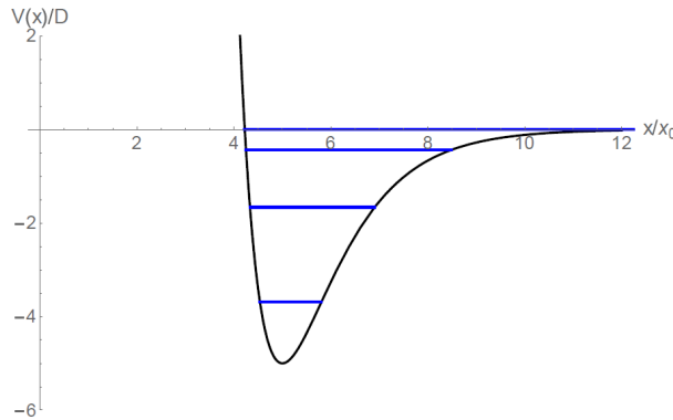
Figure 1. Morse potential
