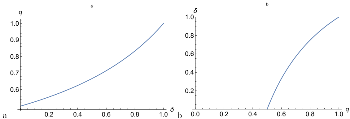
Figure 2. The relation between q and \delta : a) q on \delta , and b) \delta on q .
