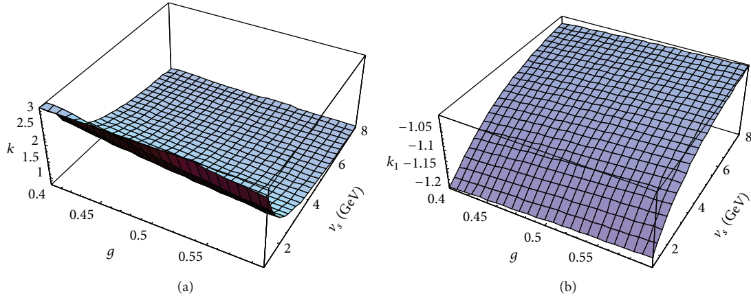
FIGURE 3: The relation between k and g, v_s provided that \delta_{\text{tree}} = 0.0005 and g \in (0.4, 0.6) , v_s \in (0, 8.0) GeV.
