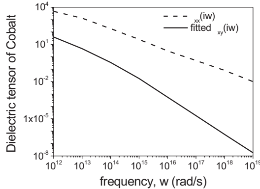
Fig. 3. The elements of the dielectric tensor of Cobalt as a function of imaginary frequency
