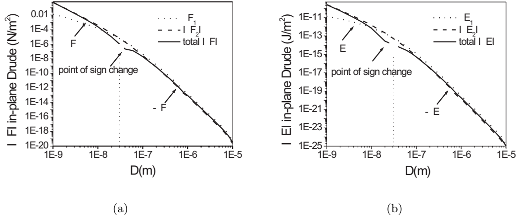
Fig. 1. Absolute of magnetic Casimir force (a) and energy (b) between the plates calculated in a Drude model for the in-plane configuration.
