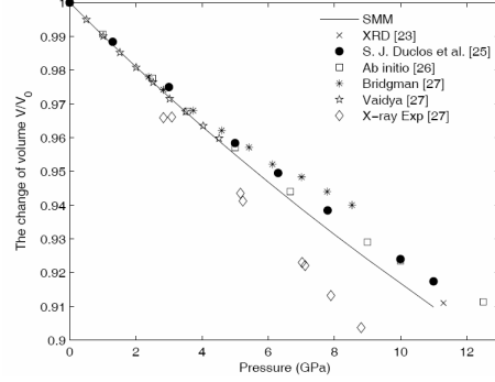
Fig. 3b. Pressure dependence of volume of Ge
