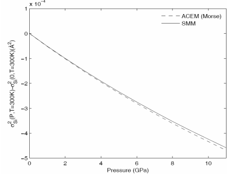
Fig. 4b. Pressure dependence of DWF of Ge
