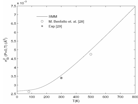
Fig. 4a. Temperature dependence of DWF of Ge
