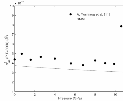
Fig. 2b. Pressure dependence of DWF of Ge
