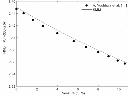
Fig. 1a. Pressure dependence of NND of Ge
