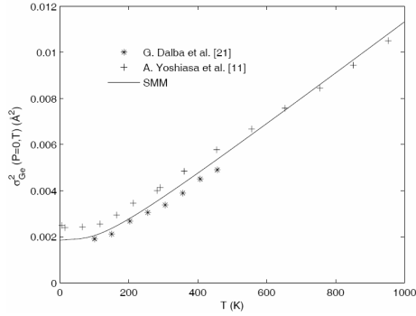
Fig. 2a. Temperature dependence of DWF of Ge
