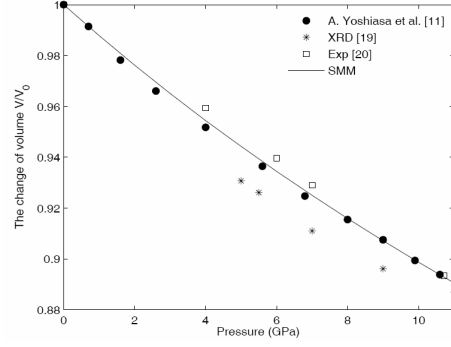
Fig. 1b. Pressure dependence of volume of Ge
