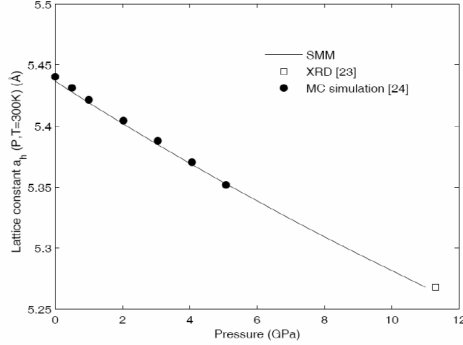
Fig. 3a. Pressure dependence of NND of Ge
