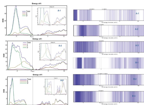
Fig. 5. Left column Density of State (DOS) of Series A NPs. Right column Spectral lines of NPs.
