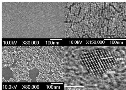
Fig. 1. SEM images of ZnO NPs synthesized following the route described in [3]. On the bottom right, HRTEM image of a NP in the [0001] direction.
