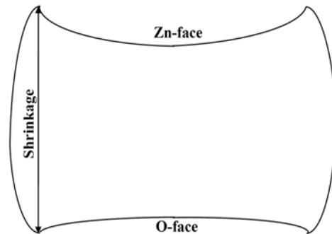
Fig. 3. Sketch of the relaxed NP shape. of studied ZnO hexagonal prismatic NP.
