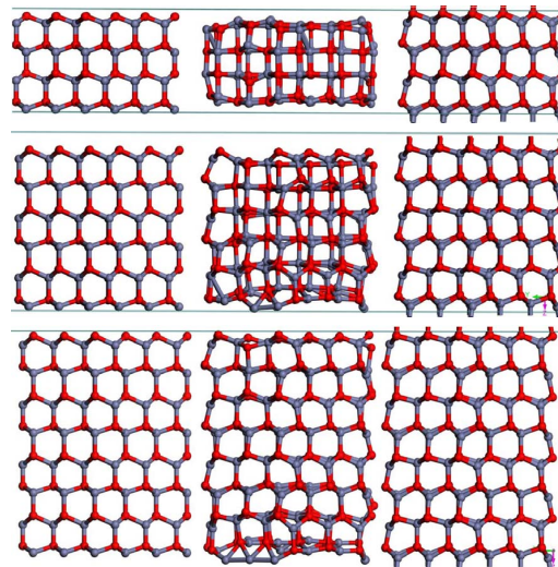
Fig. 4. (Color online) Comparable cross section view for ZnO bulk (left column), NPs (middle) and Nanowire [17] Purple axis denotes the z axis parallel to the c axis of the hcp crystal structure.
