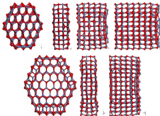
Fig. 2. (Color online) Core-shell ZnO/ZnS heterostructure NW Nanowires in [0001] direction with fully optimized structures in cross section view.
