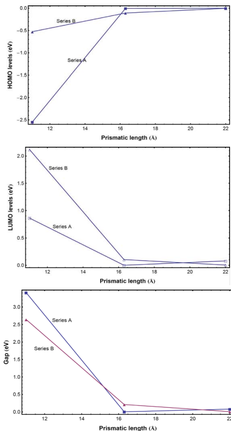
Fig. 6. HOMO, LUMO levels (Fermi level is set to zero) and energy gap of studied NPs series.
