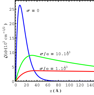
Fig. 1. The wave functions of 2DEG of an UID \text{GaN}/\text{Al}_{0.25}\text{Ga}_{0.75}\text{N} SFQW for different density of sheet of polarization charge \sigma/e .
