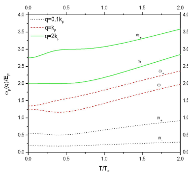
Fig. 2. The plasmon modes of DLG at several momentum values and fixed layer separation d = 100A^0 .
