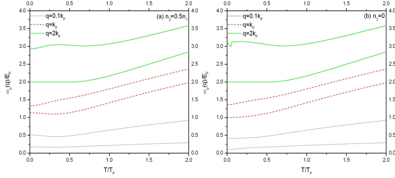
Fig. 4. The DLG plasmon modes for unequal densities at several momentum values and fixed layer separation d = 100A^0 .
