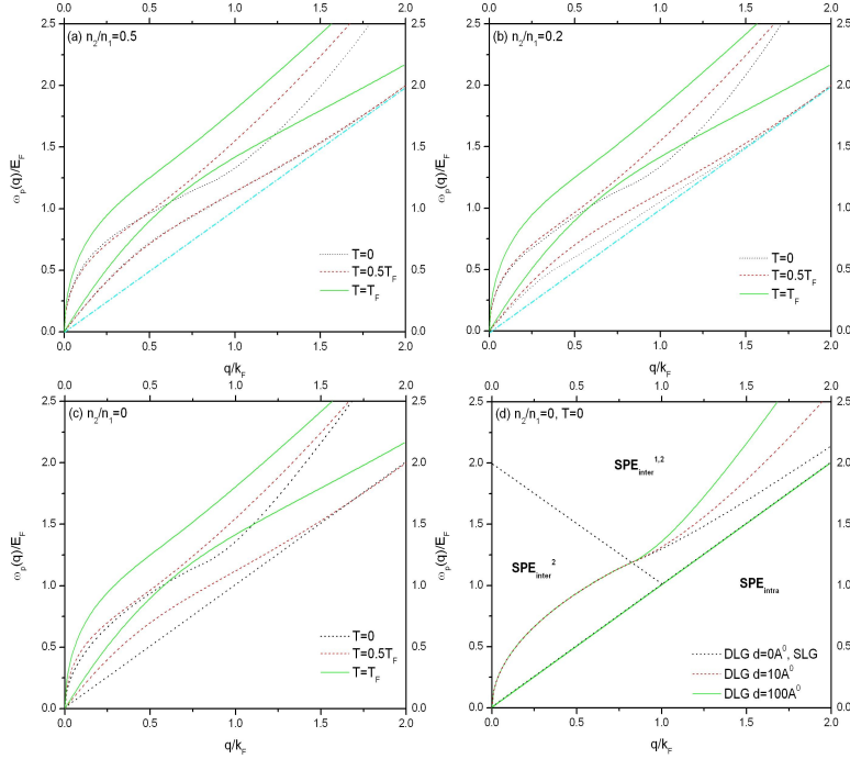
Fig. 3. Plasmon dispersions of DLG for different temperatures and layer densities. Here we use n_1 = 10^{12} \text{cm}^{-2} and d = 100 \text{\AA} .
