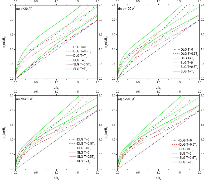
Fig. 1. Plasmon dispersions of DLG for several layer separations at T = 0 (bold dotted lines), T = 0.5T_F (bold dashed lines) and T = T_F (bold solid lines). The thin lines indicate the plasmon dispersion of SLG with the same density and temperature. Here we use the parameters: n_1 = n_2 = 10^{12} \text{cm}^{-2} and (a) d = 20 \text{Å} ( k_F d = 0.35 ), (b) d = 100 \text{Å} ( k_F d = 1.8 ), (c) d = 300 \text{Å} ( k_F d = 5.3 ) and (d) d = 500 \text{Å} ( k_F d = 8.9 ).
