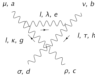
Figure 17: Four-gluon vertex (gluon-loop contribution): \Theta_{(\mu\nu)\rho\sigma}^{(ab)cdA}
