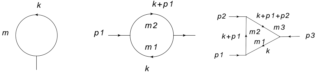
Figure 33: (a) One-point integral ; (b) Two-point integral; (c) Three-point integral.
