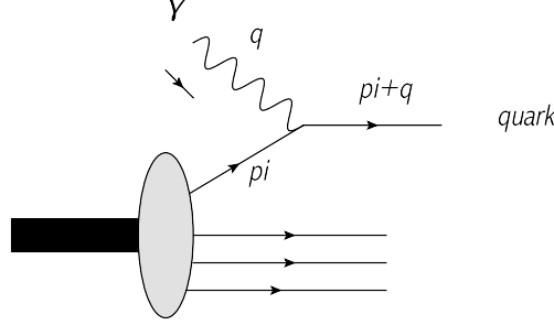
Figure 27: Deep inelastic electron-nucleon scattering in the parton model.
