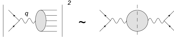
Figure 34: e^+e^- \rightarrow hadrons
