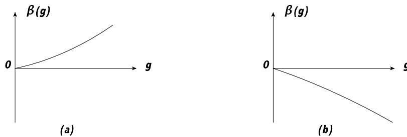
Figure 23: \beta(\bar{g}) is a monotonically (a) increasing or (b) decreasing function of \bar{g} .
