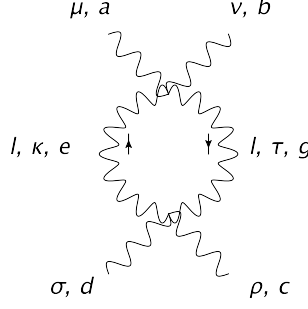
Figure 18: Four-gluon vertex (gluon-loop contribution): \Theta_{(\mu\nu)(\rho\sigma)}^{(ab)(cd)B}
