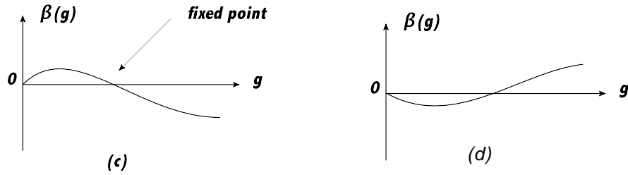
Figure 24: Other examples of the form of \beta(\bar{g}) .
