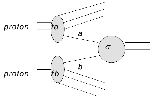
Figure 30: The hard process in pp collision
